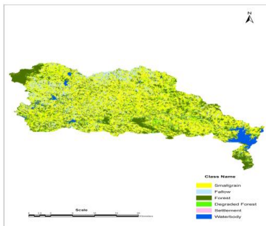
Fig.2 Landuse Map of Kumari River Basin
