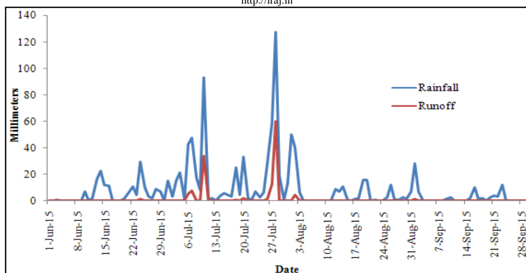
Fig4. Estimated Runoff with Daily Rainfall for Monsoon Season of 2015 of Kumari River Basin in Purulia District
