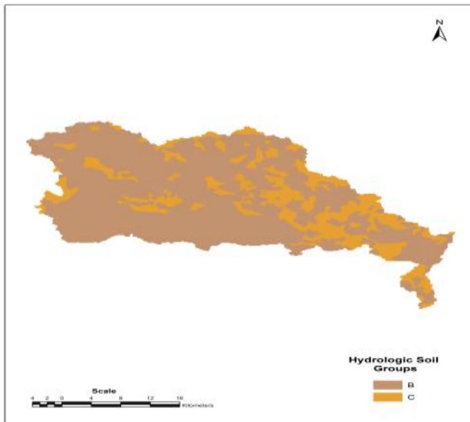
Fig.3 Hydrologic Soil Groups Map of Kumari Basin
