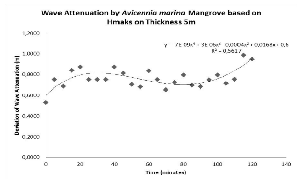
Graph 2. Wave Attenuation based on 5m thickness Hmax
