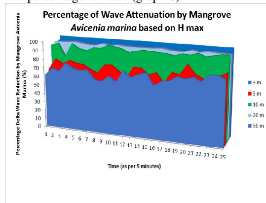
Graph 6. Percentage of Wave Attenuation by Avicennia marina Mangrove Based on H max
