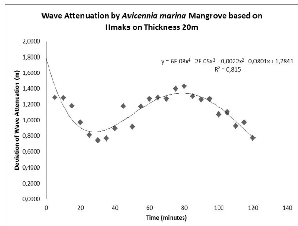
Graph 4. Wave Attenuation based on 20m thickness Hmax
