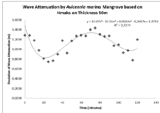
Graph 5. Wave Attenuation based on 50m thickness Hmax
