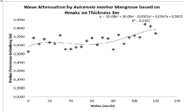
Graph 1. Wave Attenuation based on 3m thickness Hmax
