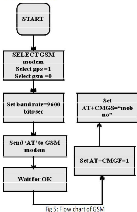
Fig.5 shows flow chart of GSM module which include the algorithm of GSM system.
